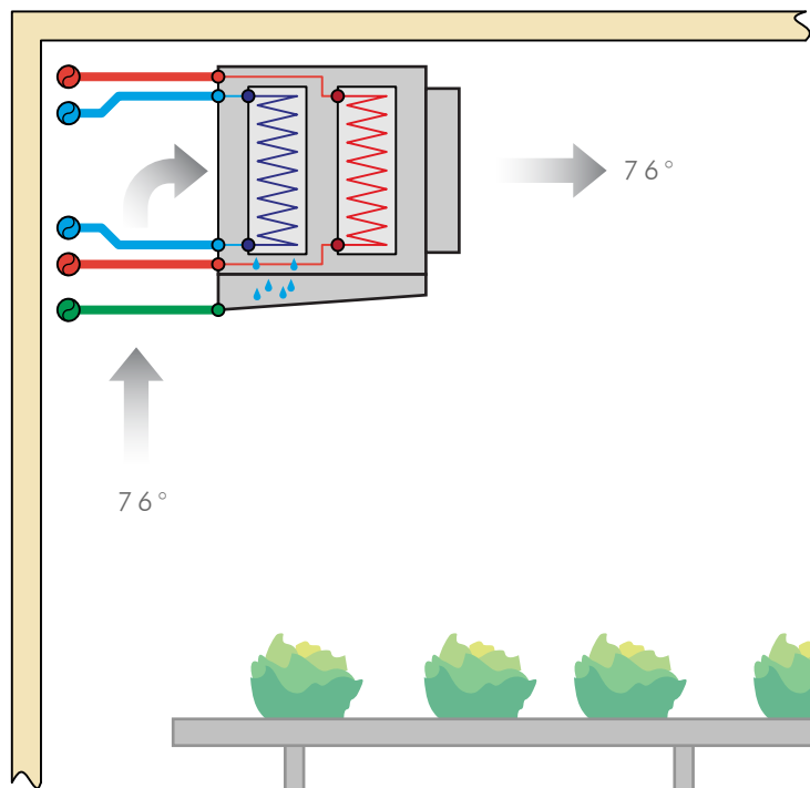
SECTION VIEW
